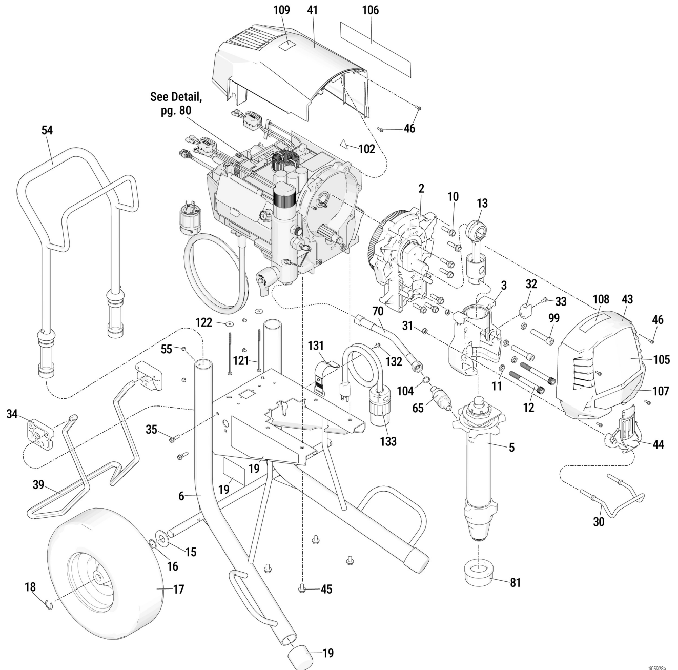
Figure 14-4: Mark XV Standard Parts Diagram
