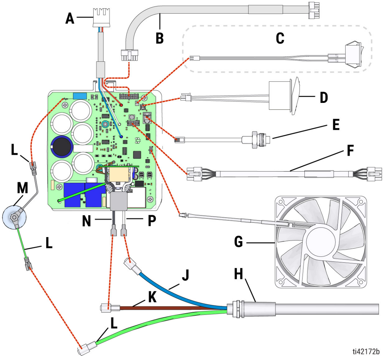
Figure 16-2: Wiring Diagram for 110 V UK
