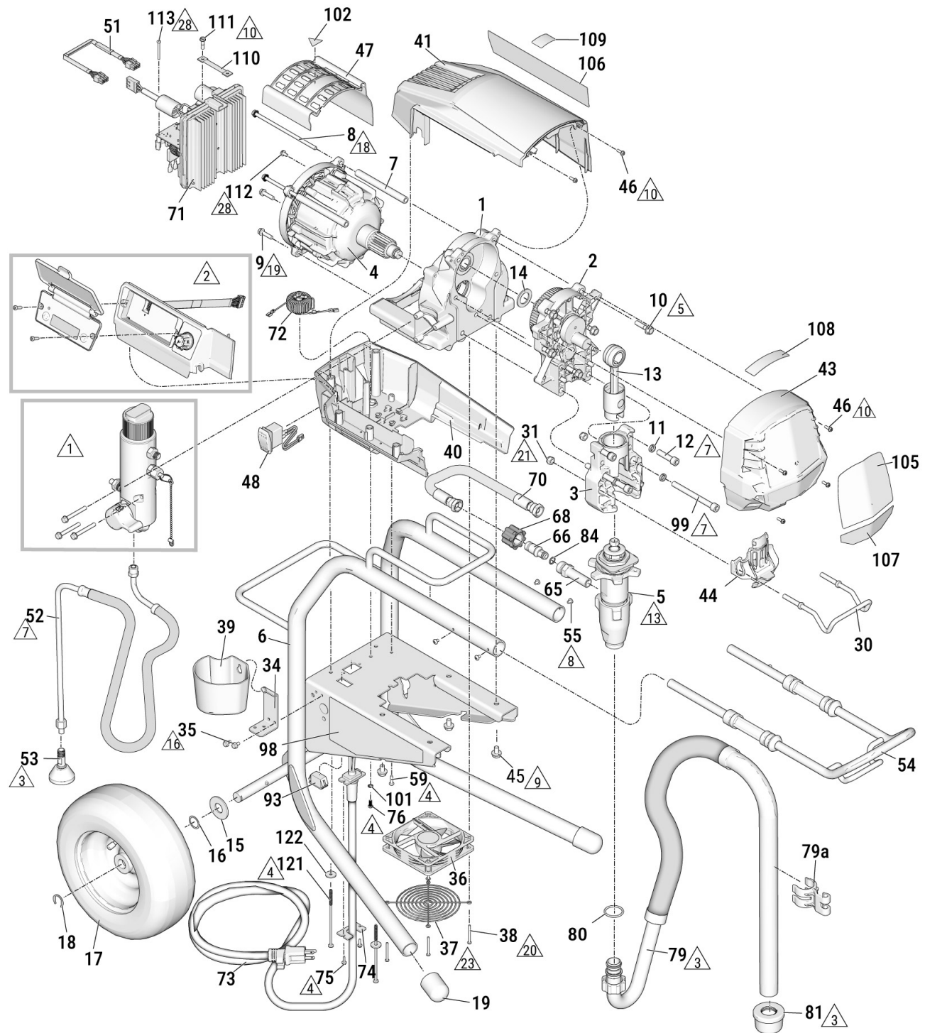
Figure 14-1: 695 XT Lo-Boy Parts Diagram
