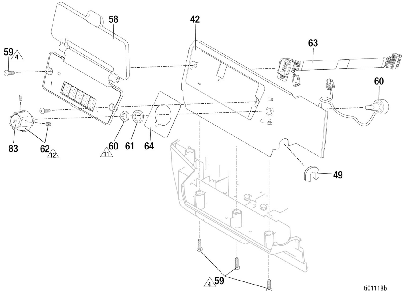
Figure 14-13: Digital Display Parts Diagram
