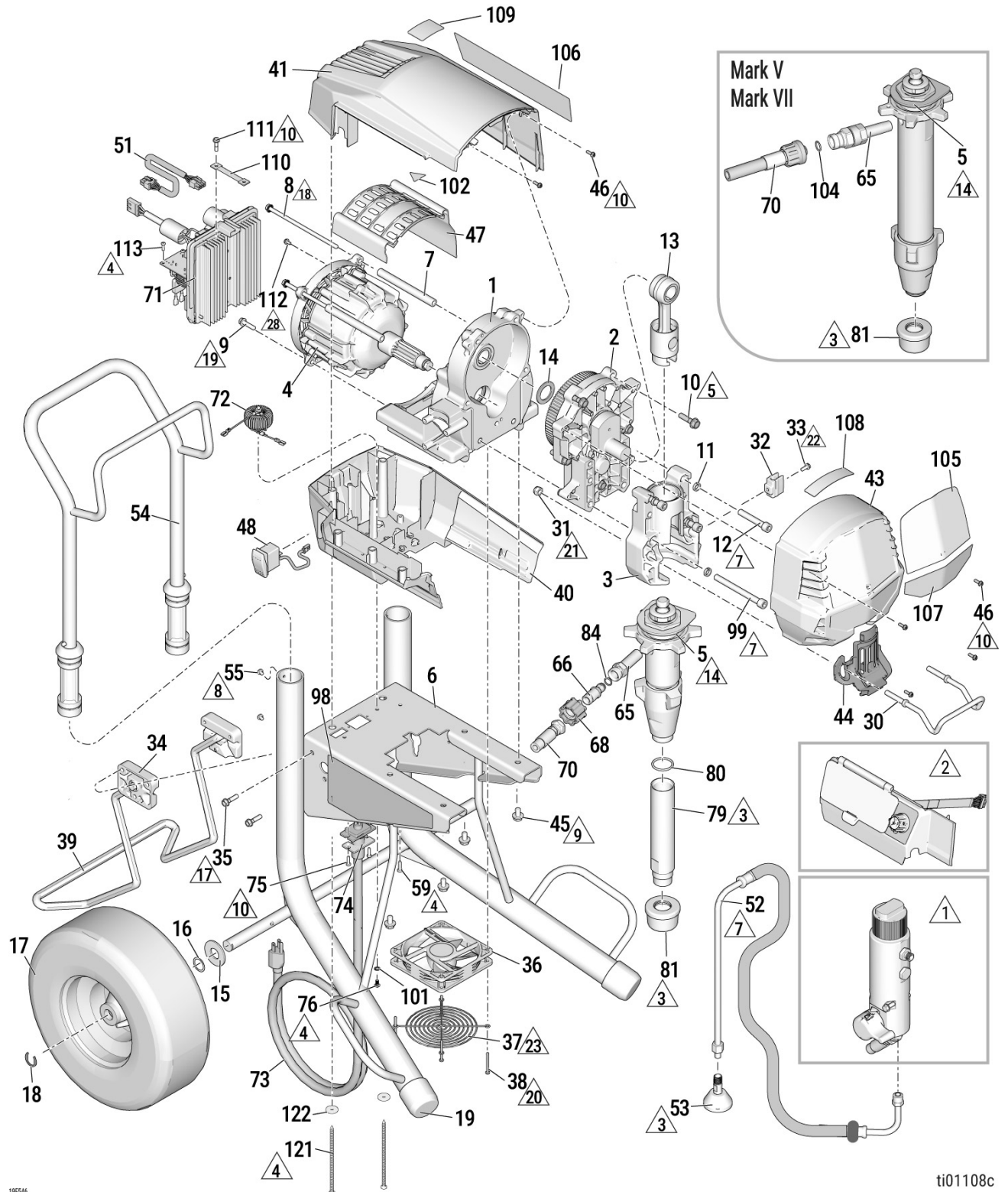
Figure 14-3: 1095 XT, Mark V, Mark VII Standard Hi-Boy Parts Diagram
