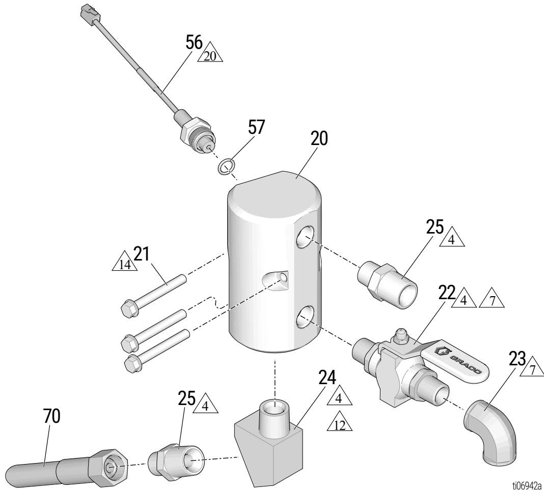
Figure 14-12: Mark HP Filter Parts Diagram
