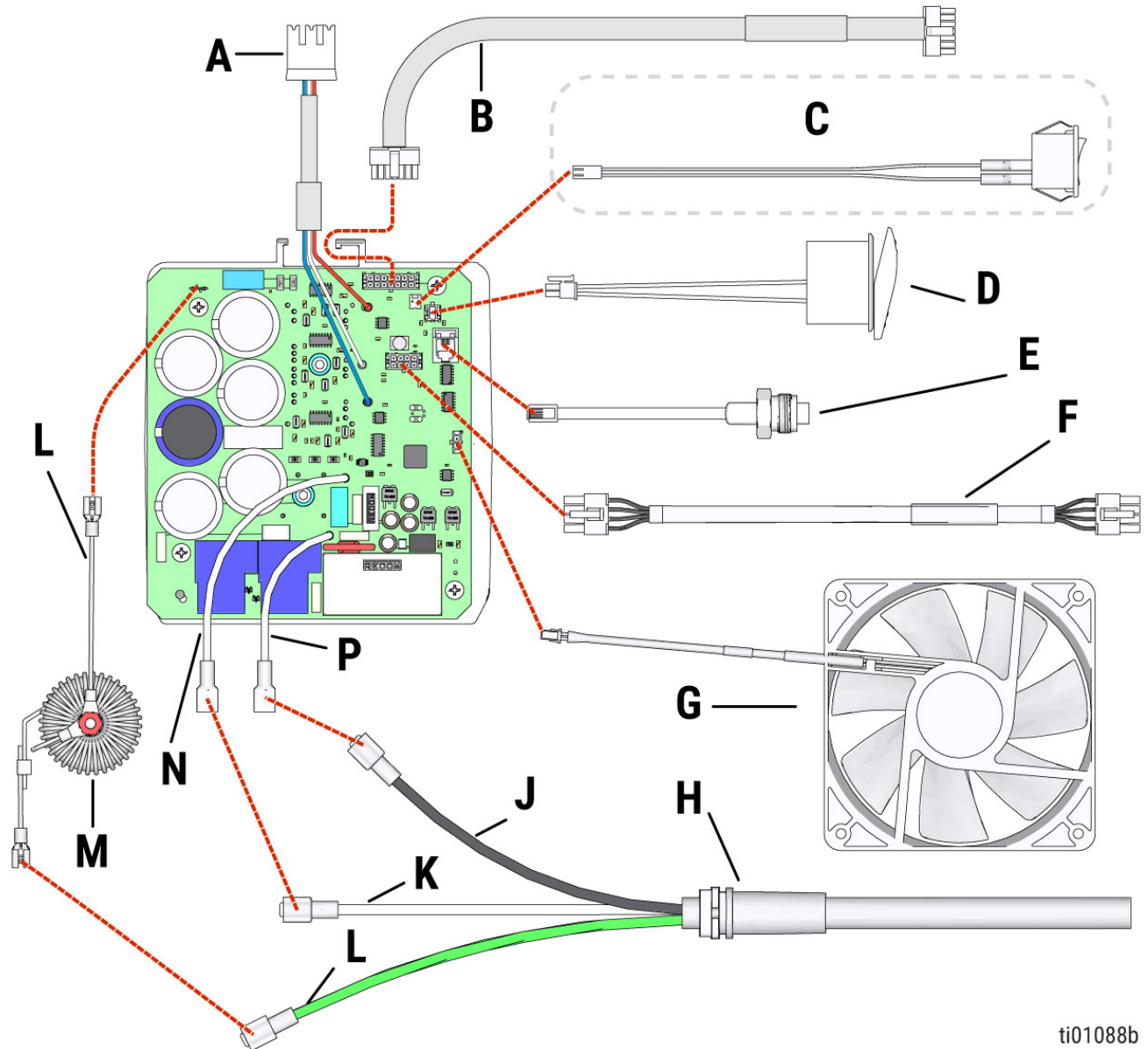
Figure 16-1: Wiring Diagram for 110-120 V
