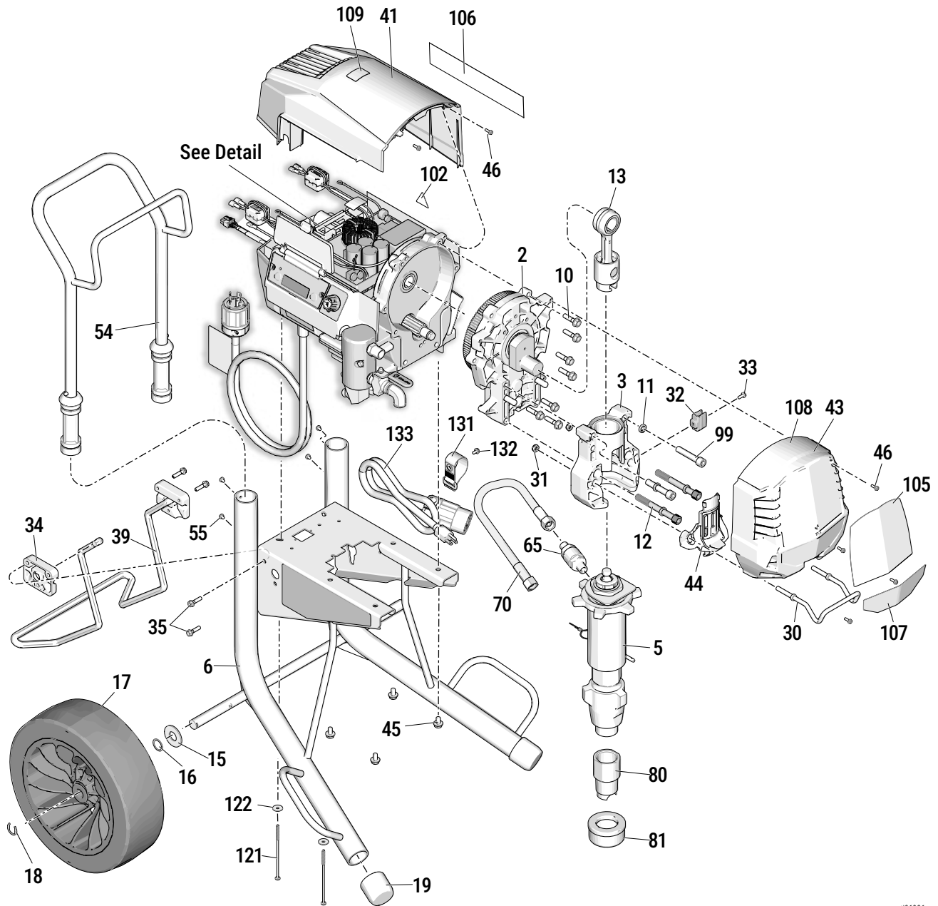
Figure 14-7: Mark HP Parts Diagram
