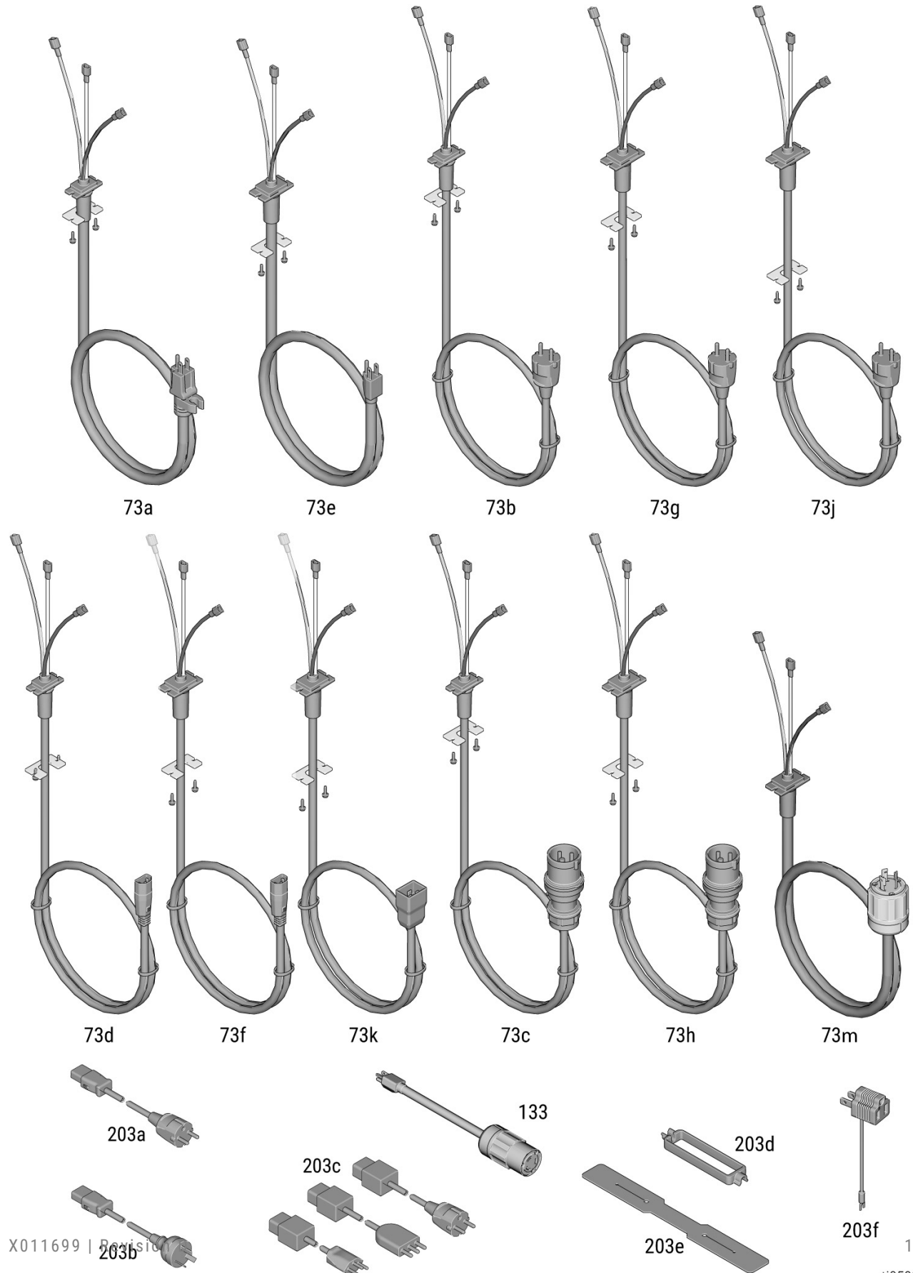
Figure 14-15: Power Cord Parts Diagram
