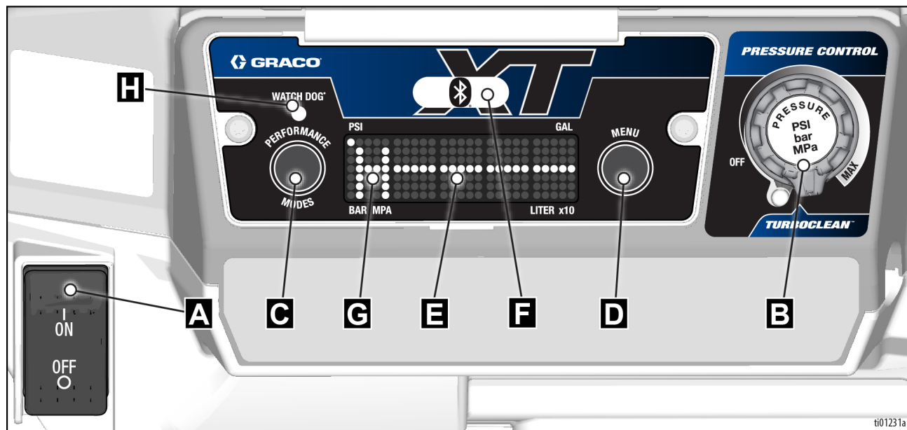
Figure 6-5: Components for Controls and Display
