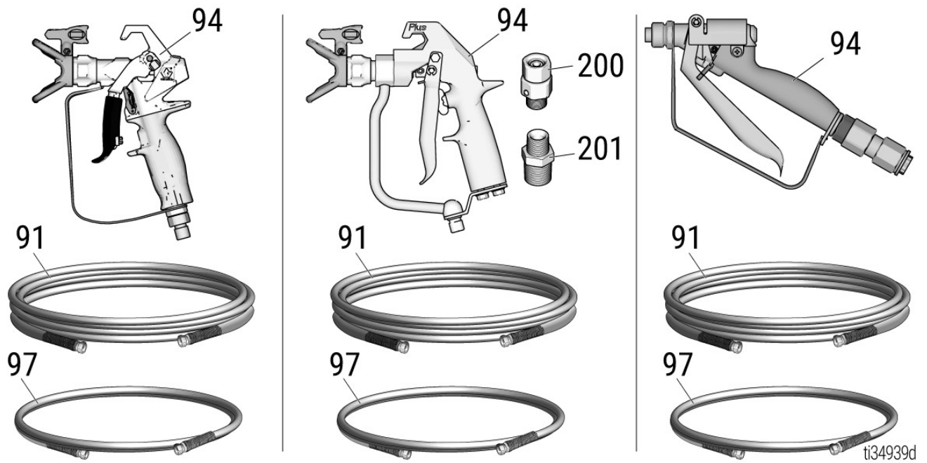
Figure 14-14: Spray Gun and Hose Parts Diagram
