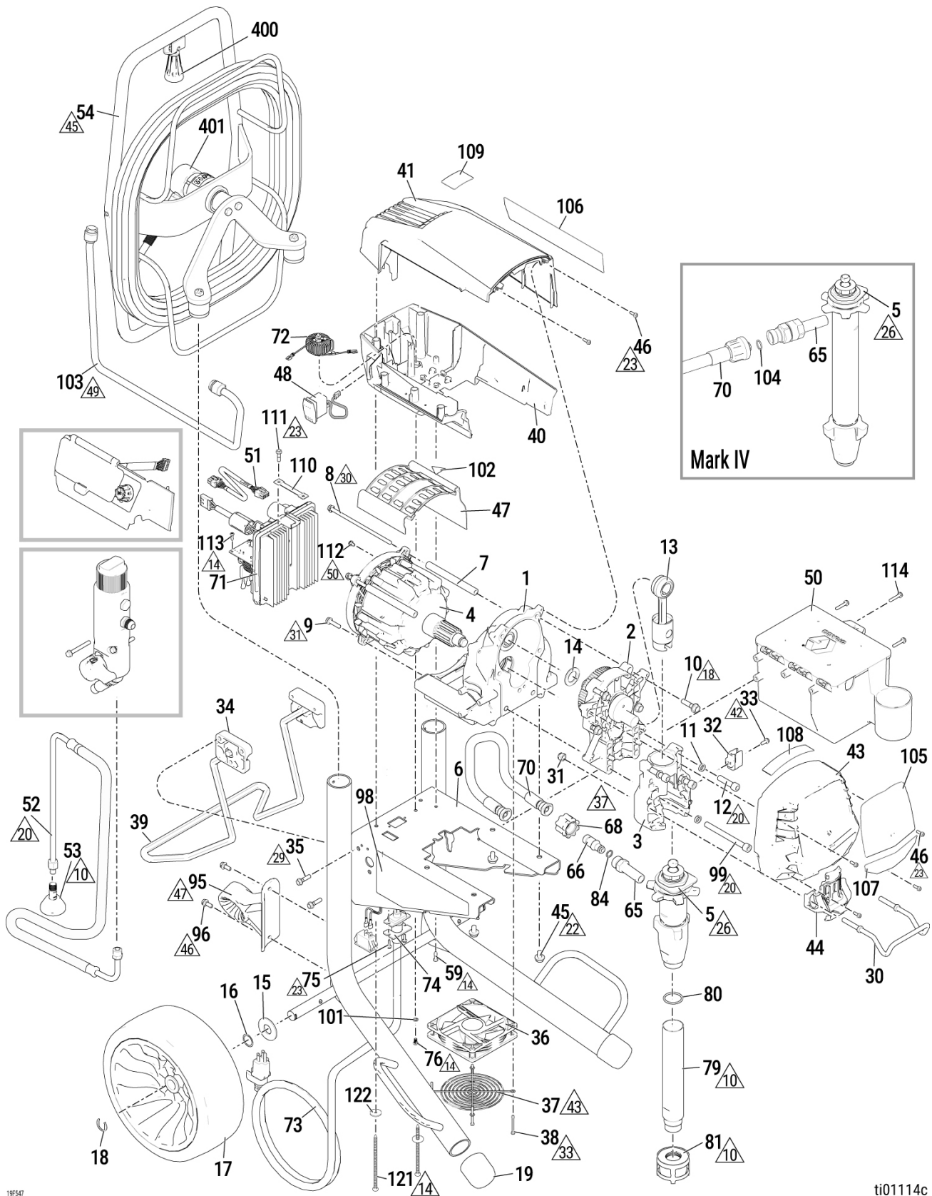
Figure 14-9: 695 XT, 795 XT, Mark IV Pro Hi-Boy Parts Diagram
