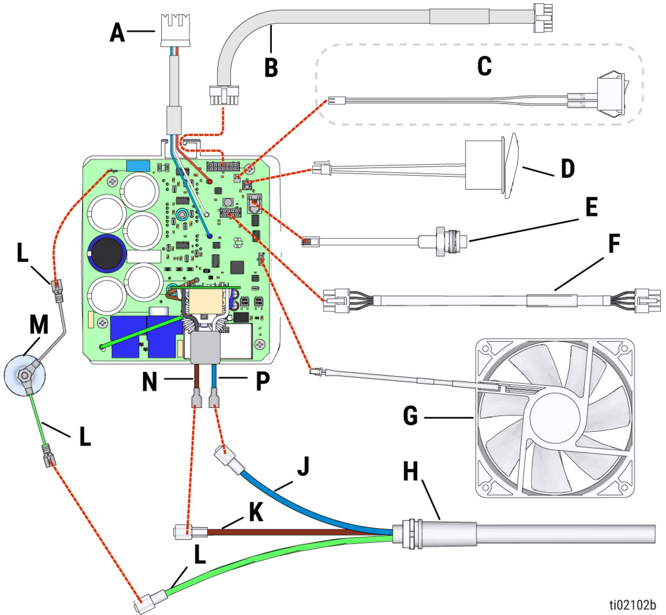
Figure 16-3: Wiring Diagram for 220-240 V
