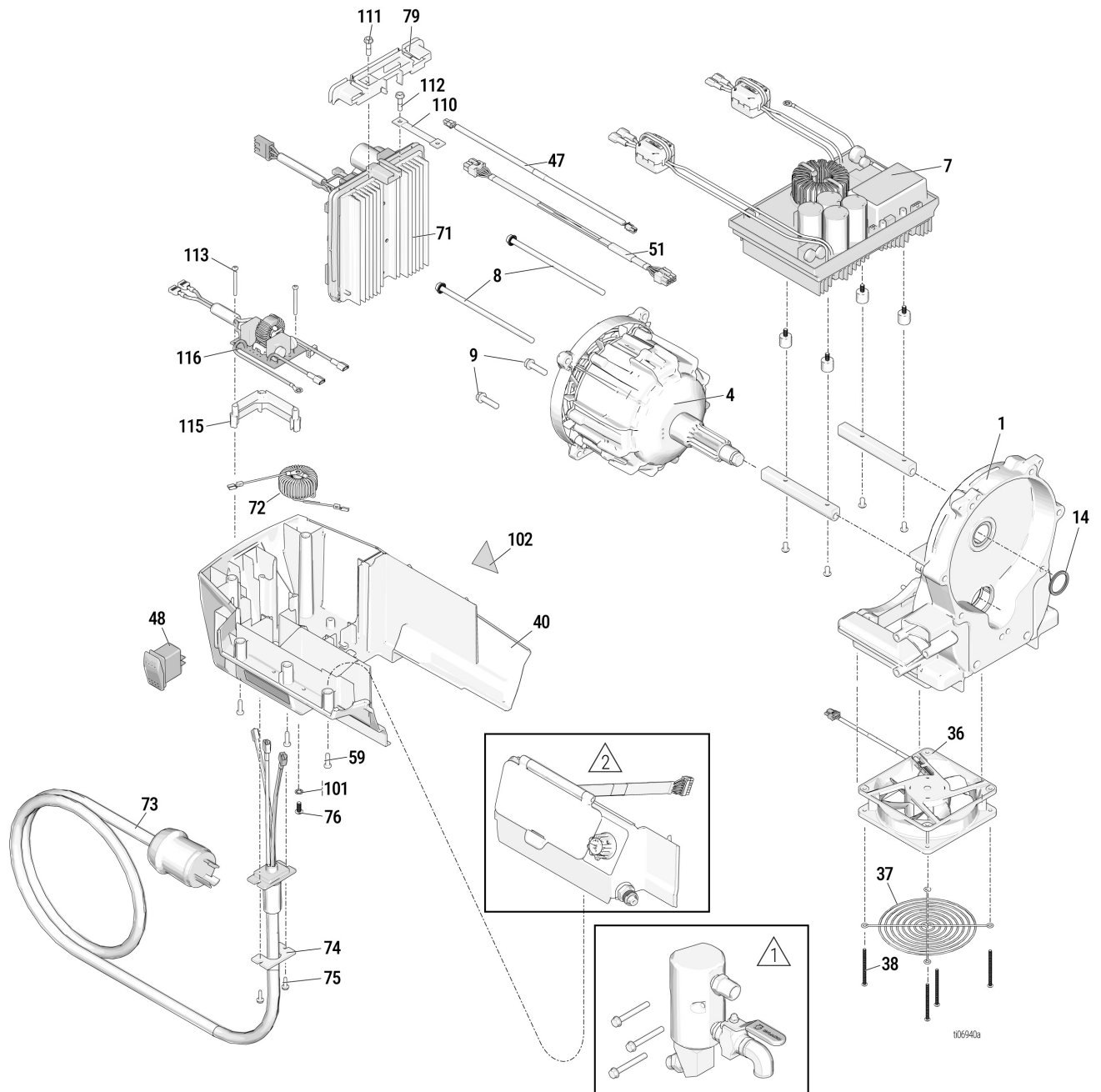
Figure 14-8: Enlarged Housing and Motor Diagram
