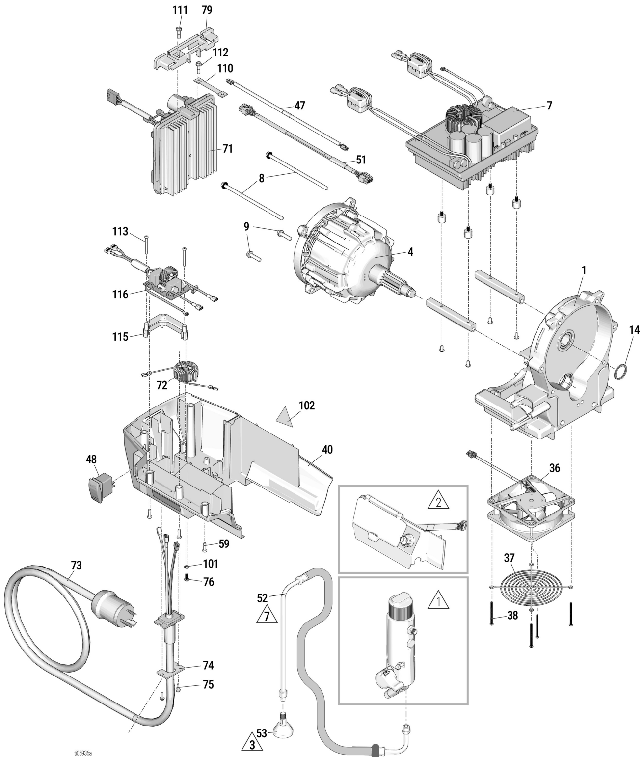
Figure 14-5: Enlarged Housing and Motor Diagram
